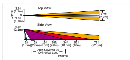
VERTICAL BARRIER LENS (P/N D 03)
